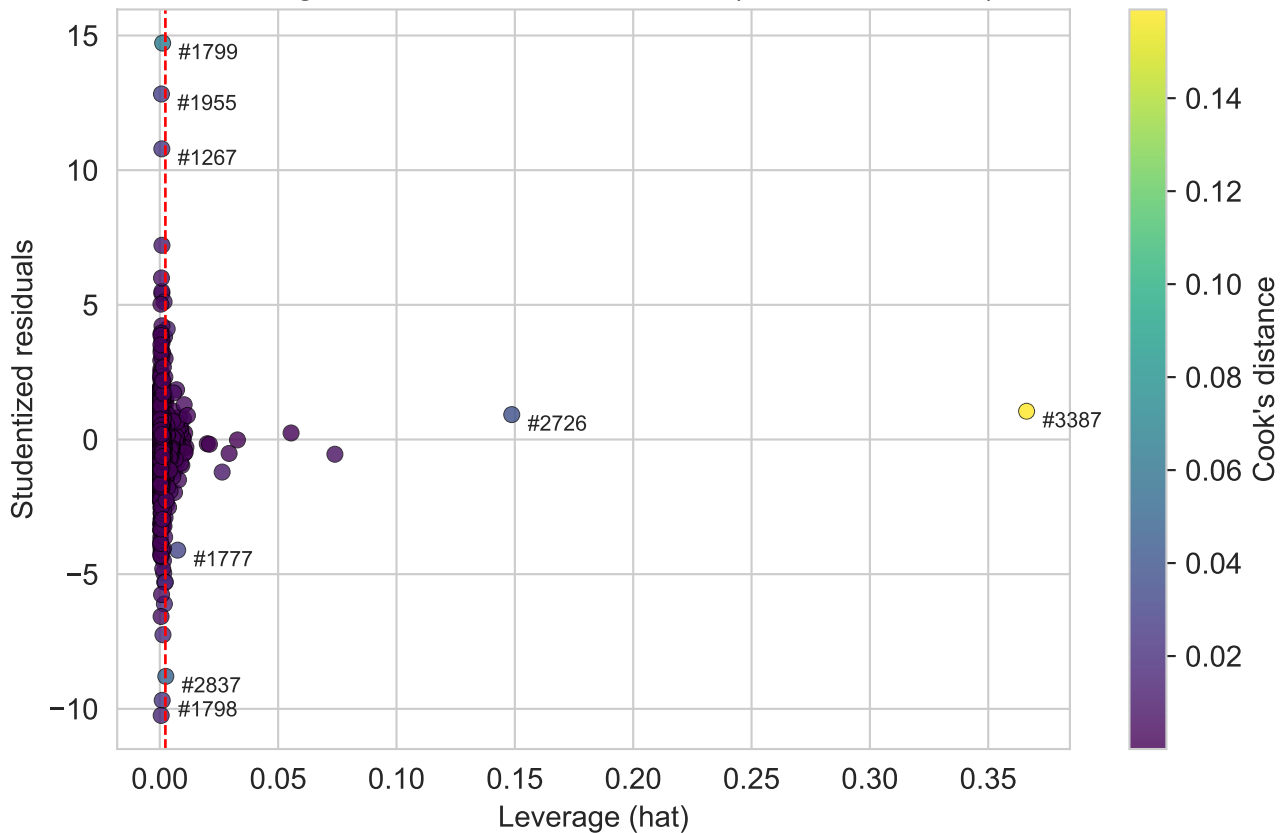
Leverage vs Studentized residuals (Cook's distance)
