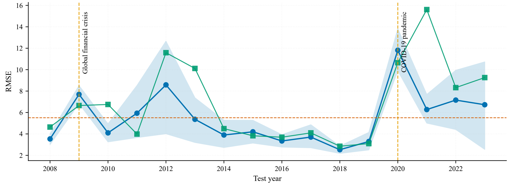
RMSE by test year (h=3)
