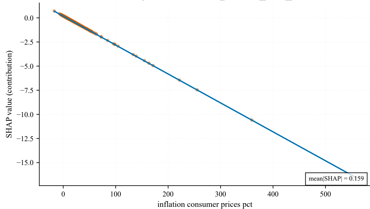
SHAP dependence — inflation_consumer_prices_pct
