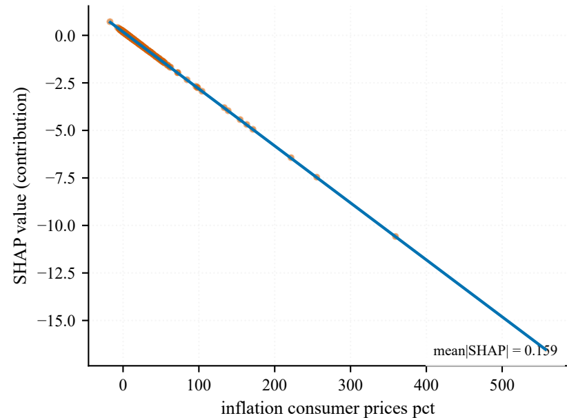
SHAP dependence — inflation_consumer_prices_pct
