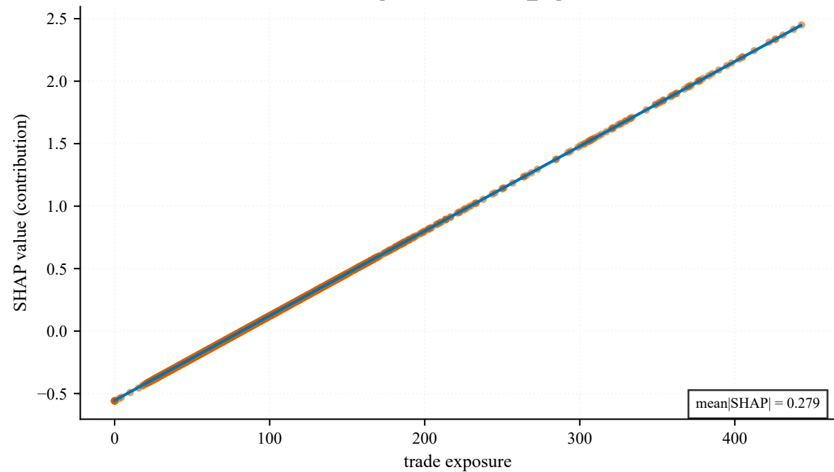
SHAP dependence — trade_exposure
