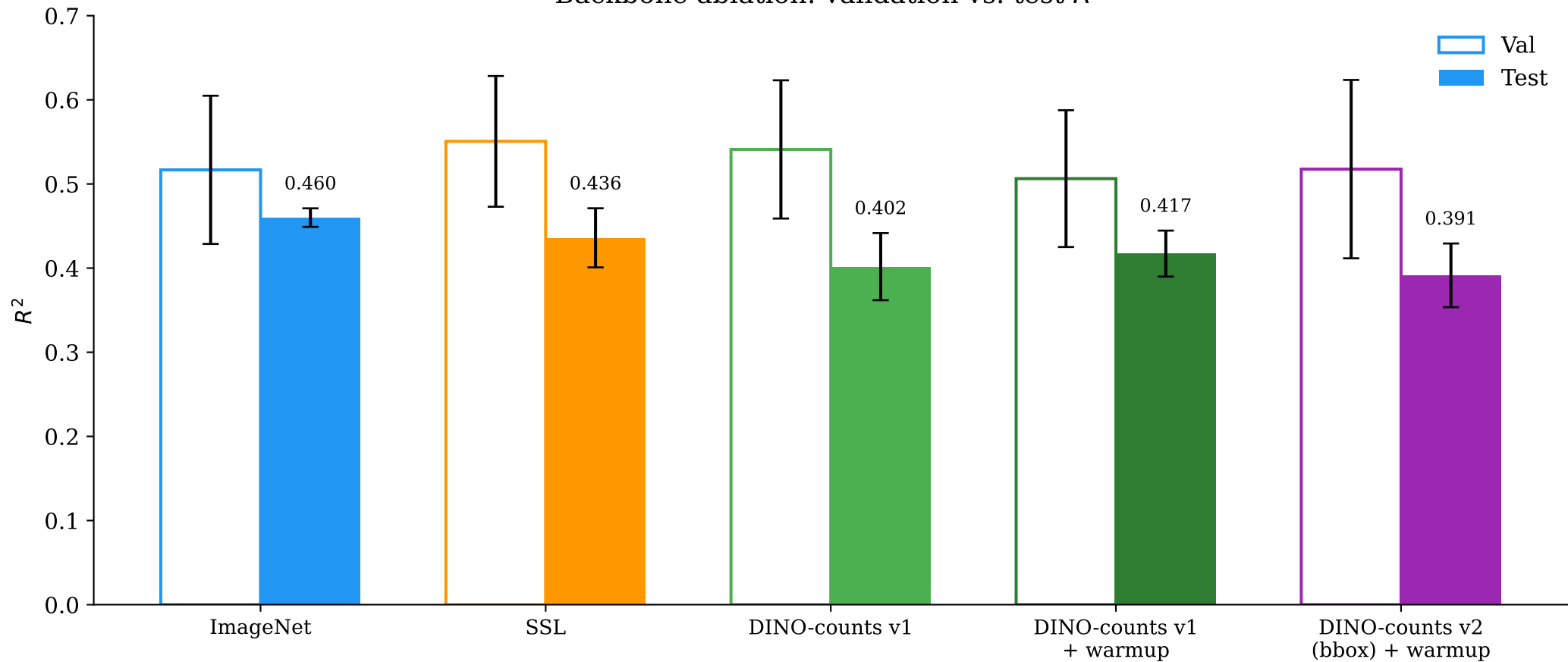
Backbone ablation: validation vs. test R^2
