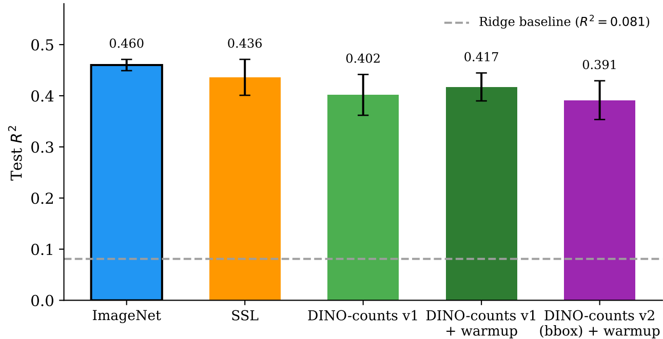
Brightness prediction R^2 by backbone initialisation
