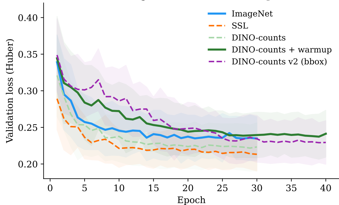
Fine-tuning validation loss over epochs
