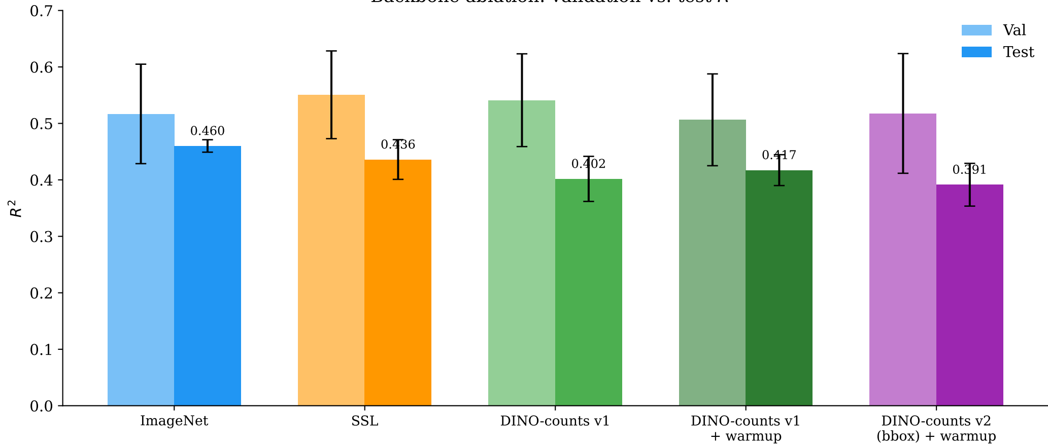
Backbone ablation: validation vs. test R^2
