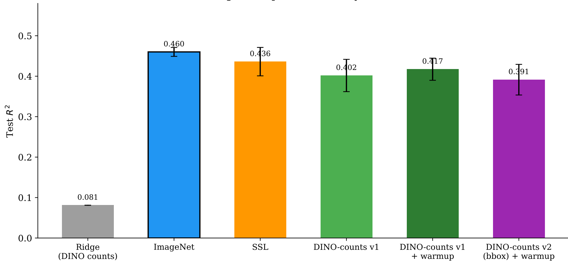
Brightness prediction R^2 by model
