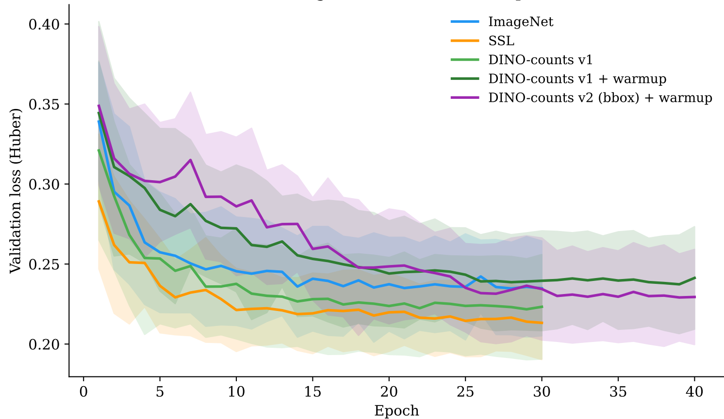
Fine-tuning validation loss over epochs
