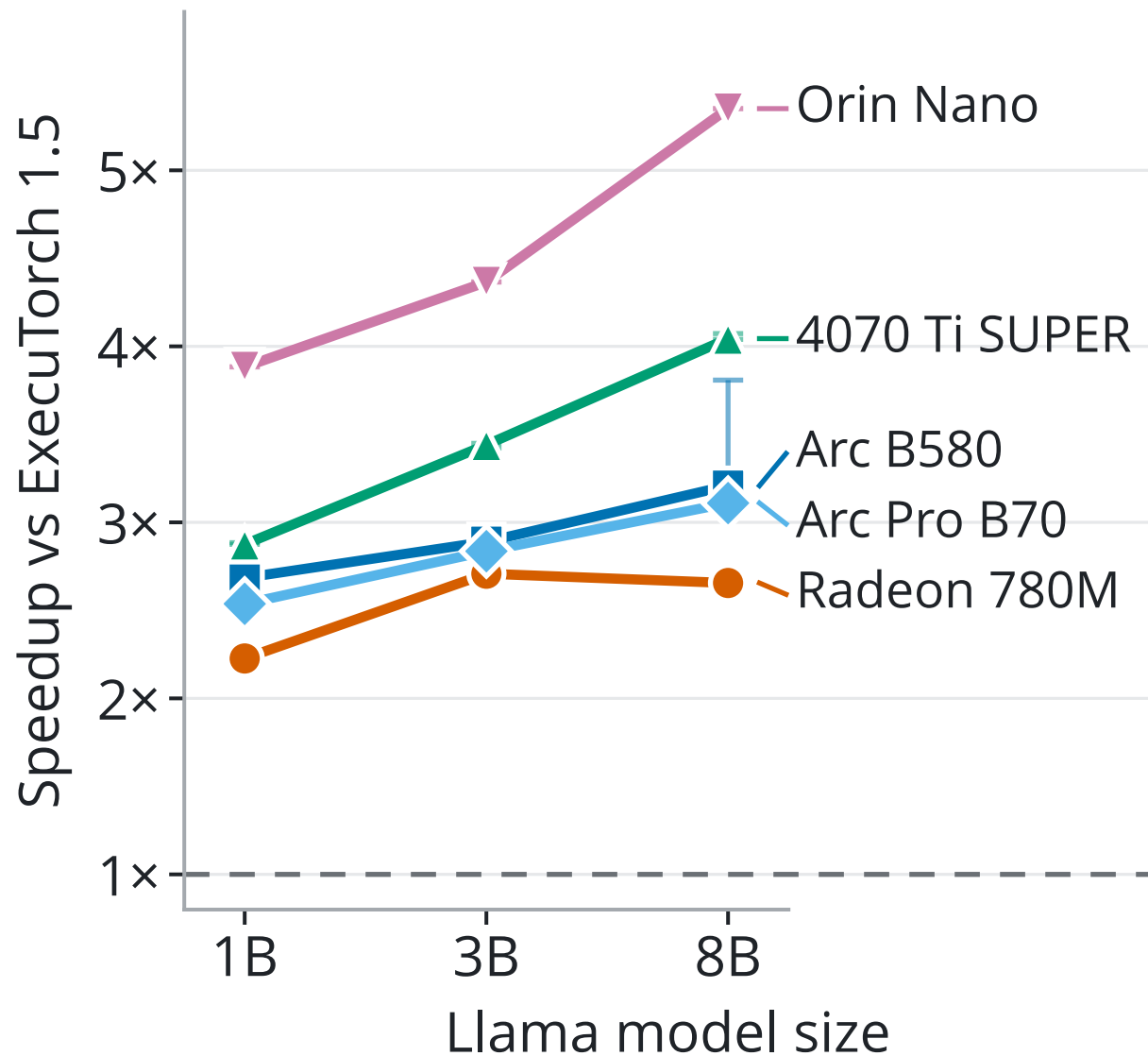
4-bit weights
