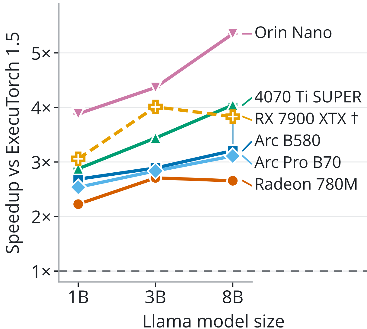
4-bit weights
