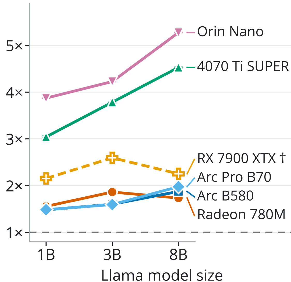
8-bit activations + 4-bit weights
