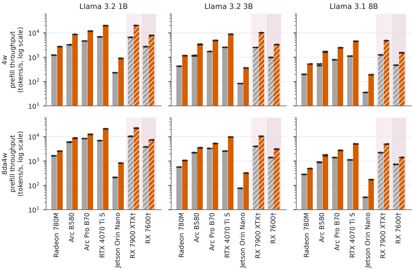
2048-token prompt, ExecuTorch Vulkan (llama_main). Bars: median; whiskers: min-max of n=5 runs; dots: individual runs. † pre-release (RX 7900 XTX, RX 7600): SARC rows unverified (ET_VK_SARC_UNVERIFIED=1); different .pte export, so absolute tok/s are not strictly comparable; drivers: AMDVLK (RX 7900 XTX), RADV Mesa 26.2.3 (RX 7600).
