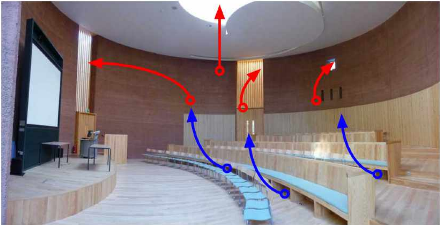
Shepard theatre with natural ventilation controls. A large open curved lecture theatre. Figure.....58
