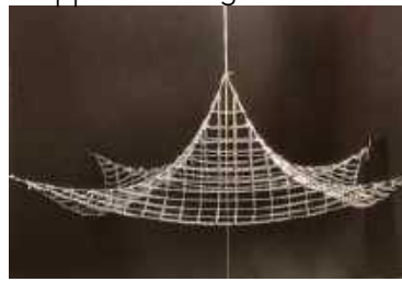
Figure.....14: Chain model
