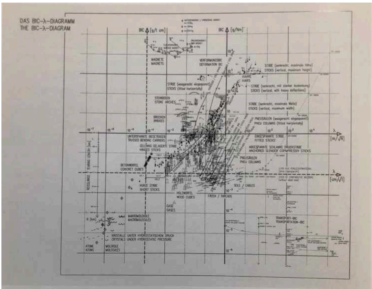
Figure.....17: BIC diagram to assess lightweight use of different structures BIC = m / Tra . Tra was used to classify structural forms. Tr = Ti / Ta . Ti is the product of force and distance and Ta is the product of all external loads and the distance from the supports. \lambda = s / \sqrt{F} is the relative slenderness formula
