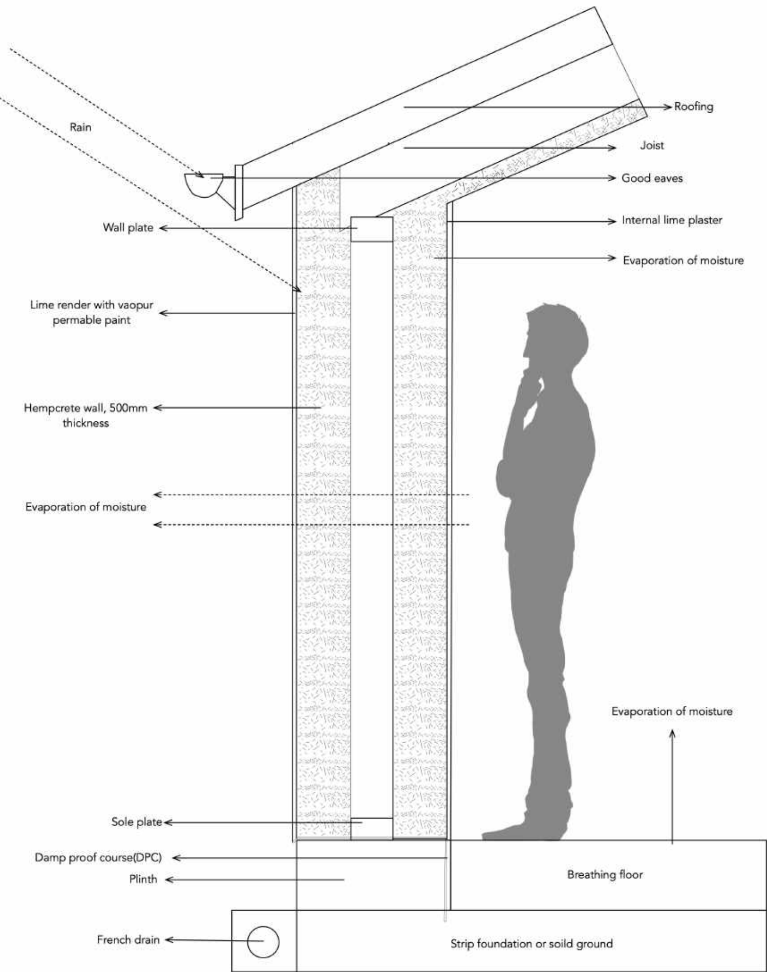
Figure.....46: Breathable wall works by allowing evaporation between the hurts and the binder within the wall, the hygroscopic nature leads to moisture control which ensures no mold build up occurs
