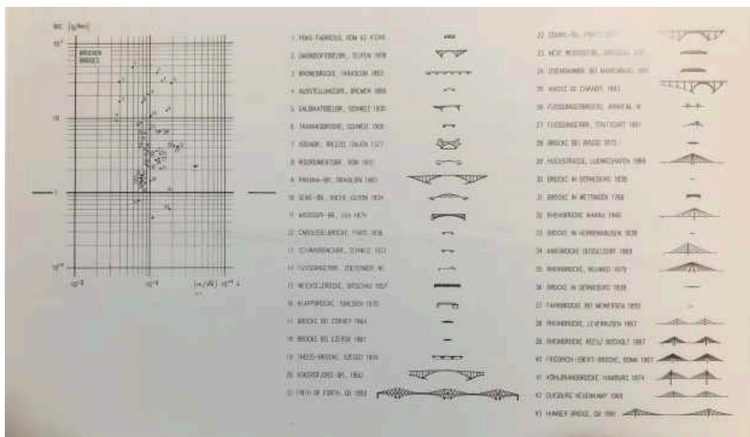
Figure.....18: BIC diagram used in bridge constructions
