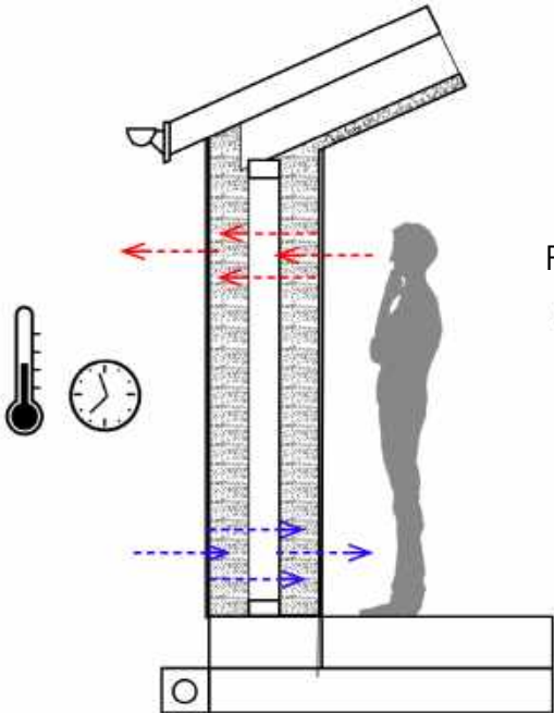
Figure.....48: Slow release of hot and cold air
