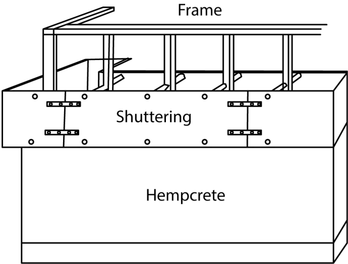
Figure.....39: Shuttering to build the wall which is built in stages allowing it to dry
