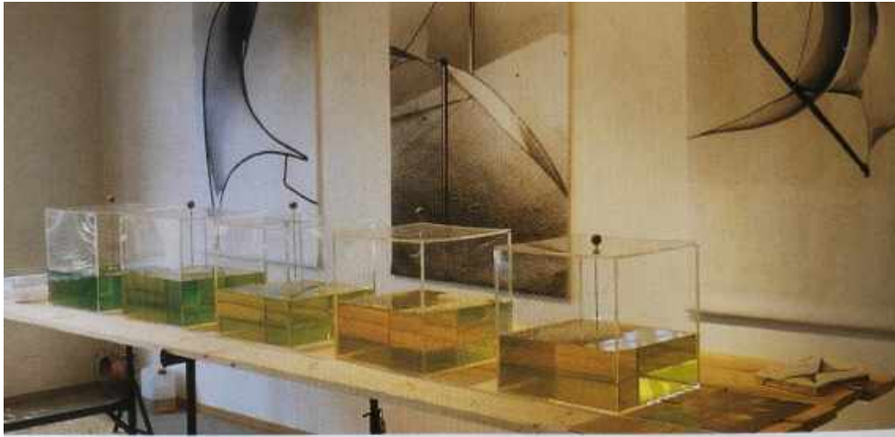
Figure.....10 Soap film membranes to produce minimal areas as form finding models for tension loaded constructions
