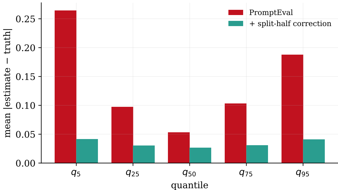
Split-half correction cuts MMLU tail error ~82% (budget=200)
