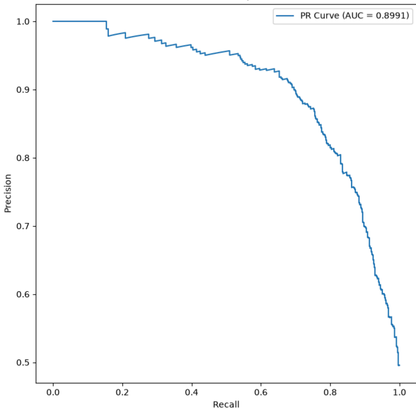
Precision-Recall Curve (Visu Wavelet Dataset, Contractive Autoencoder, Gaussian \chi^2 Error Function)
