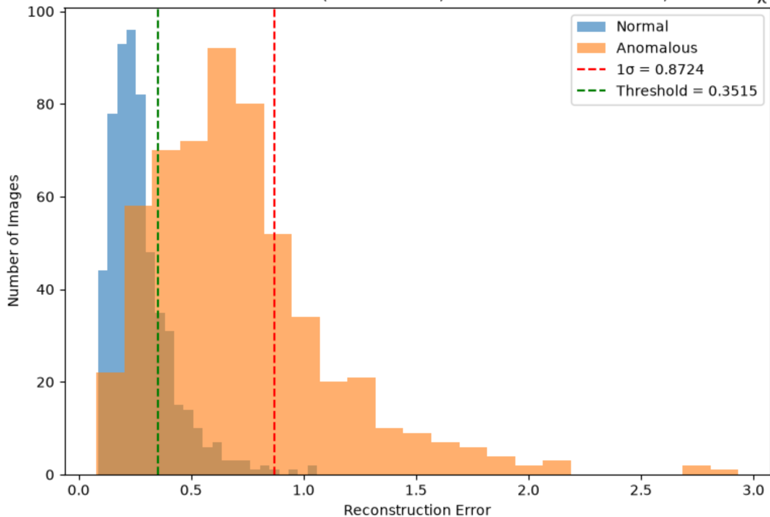
Distribution of Reconstruction Errors (Visu Wavelet, Contractive Autoencoder, Gaussian \chi^2 Error)
