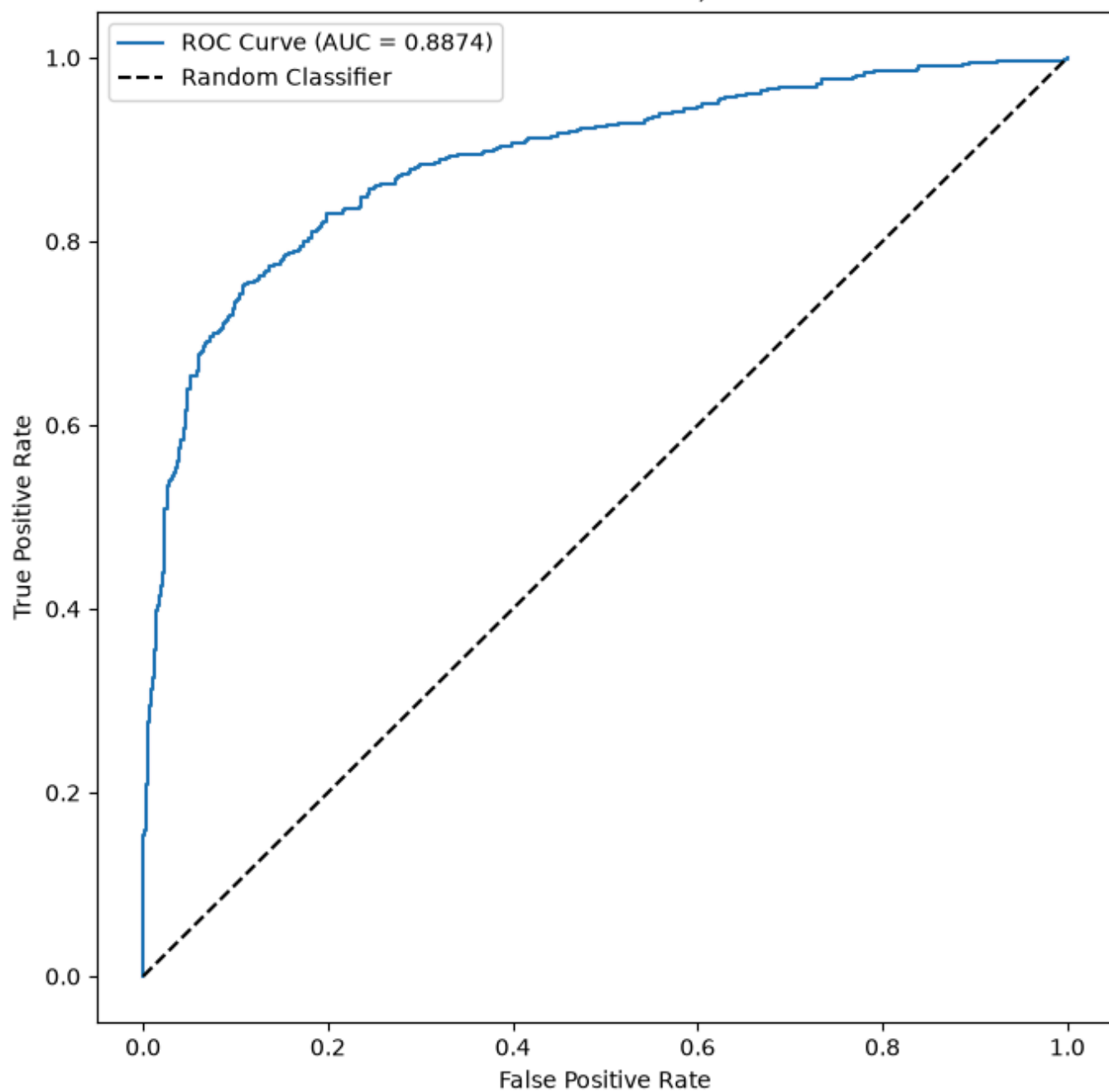
Receiver Operating Curve (Visu Wavelet Dataset, Contractive Autoencoder, Gaussian \chi^2 Error Function)
