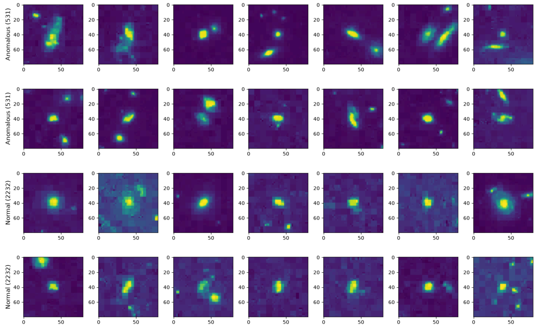
Predictions made by Visu Wavelet, Contractive Autoencoder, Gaussian \chi^2 Error
