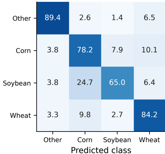
a Test confusion matrix
