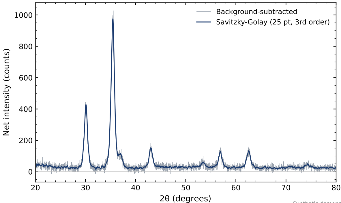
Figure 2. Background-subtracted synthetic XRD pattern
