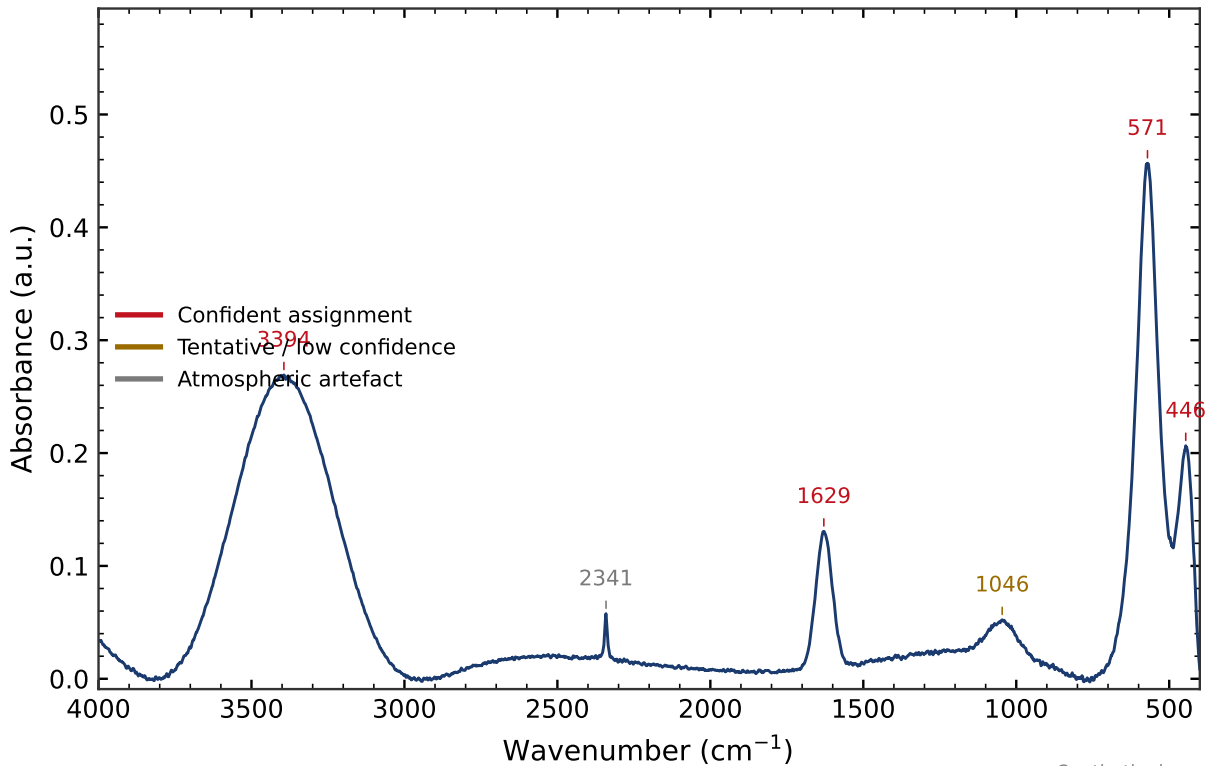
Figure 8. Band-labelled synthetic FTIR spectrum
