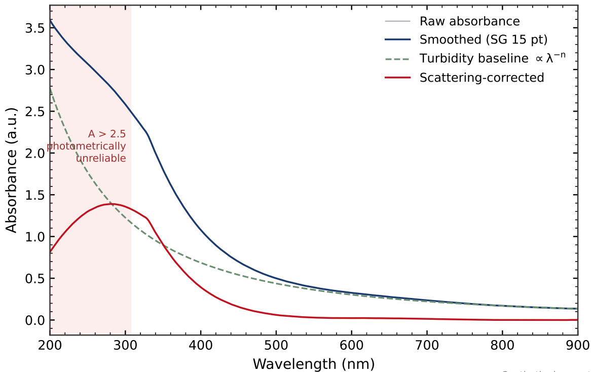
Figure 9. Synthetic UV-Vis spectrum of an aqueous \text{Fe}_3\text{O}_4 dispersion
