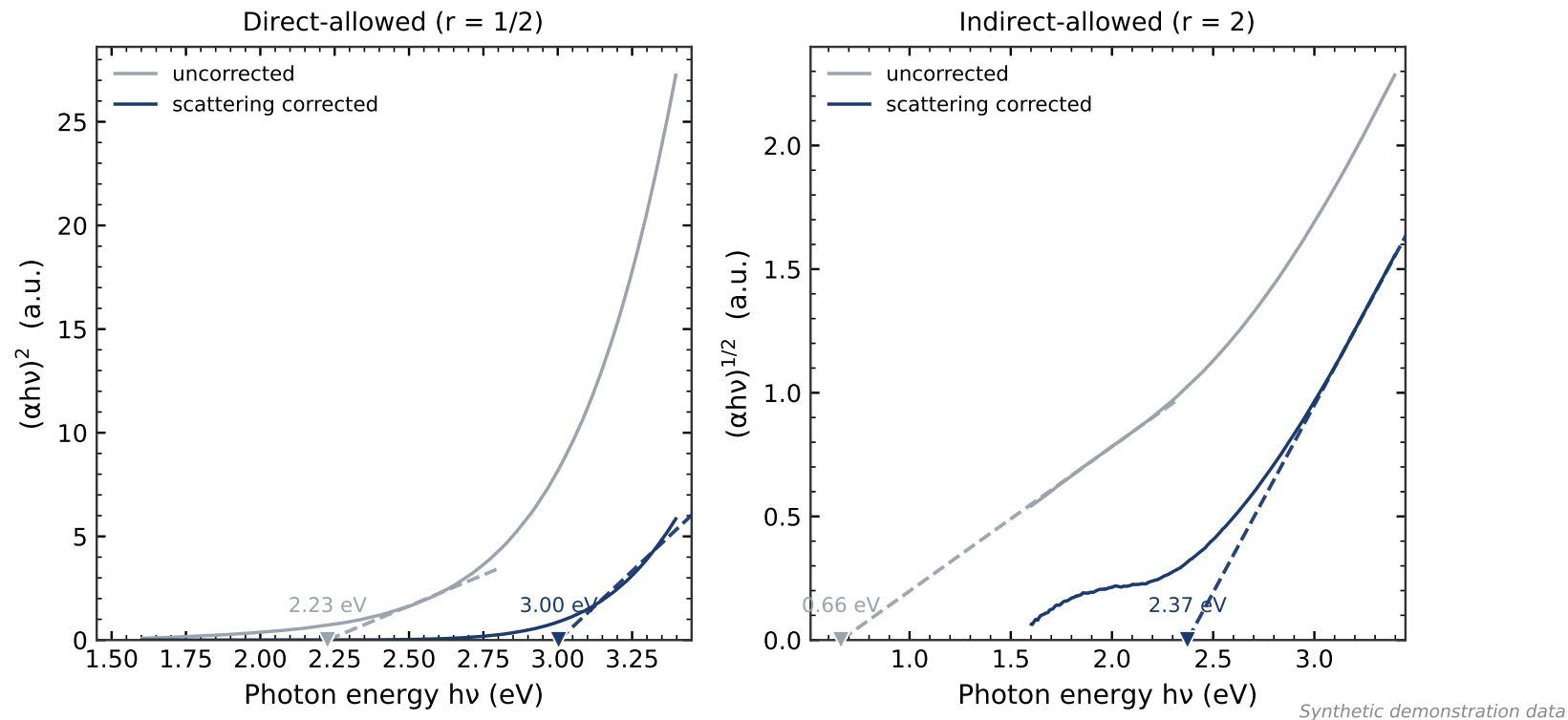
Figure 10. Tauc analysis shown as a METHOD DEMONSTRATION -- the extracted values are not a band gap of \text{Fe}_3\text{O}_4
