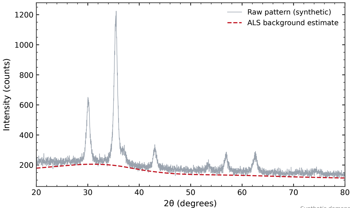
Figure 1. Raw synthetic XRD pattern of \text{Fe}_3\text{O}_4 with estimated background
