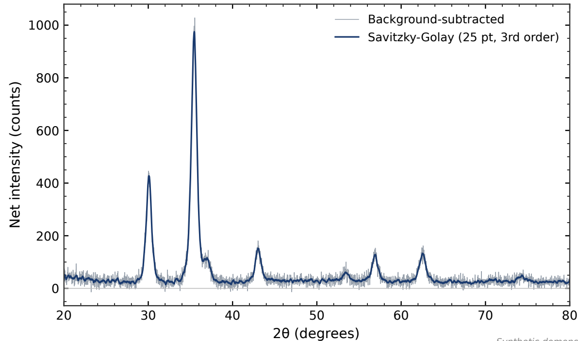
Figure 2. Background-subtracted synthetic XRD pattern
