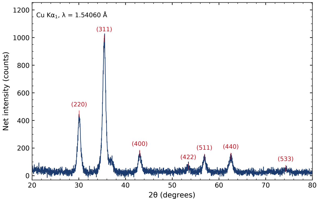
Figure 3. Indexed synthetic XRD pattern (cubic \text{Fe}_3\text{O}_4 , \text{Fd}\bar{3}\text{m} )
