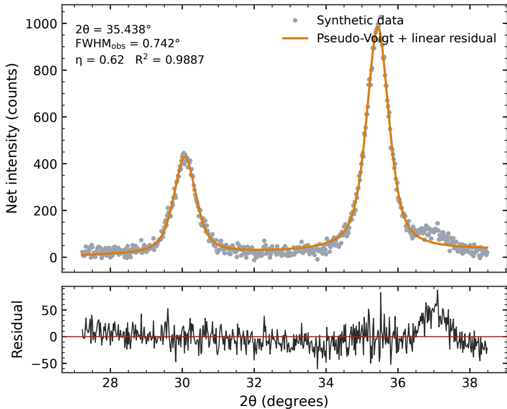
Figure 4. Pseudo-Voigt profile fit to the (311) reflection
