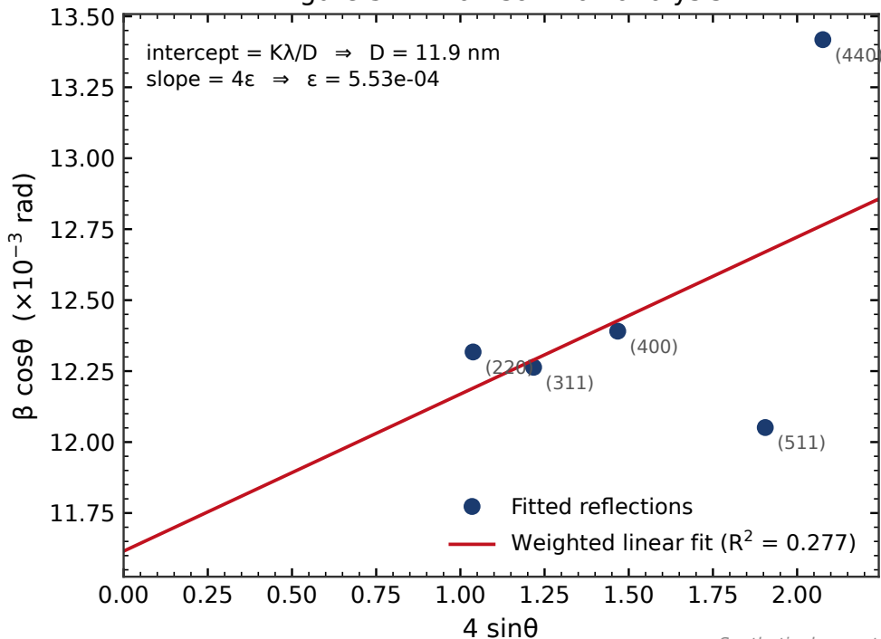
Figure 5. Williamson-Hall analysis
