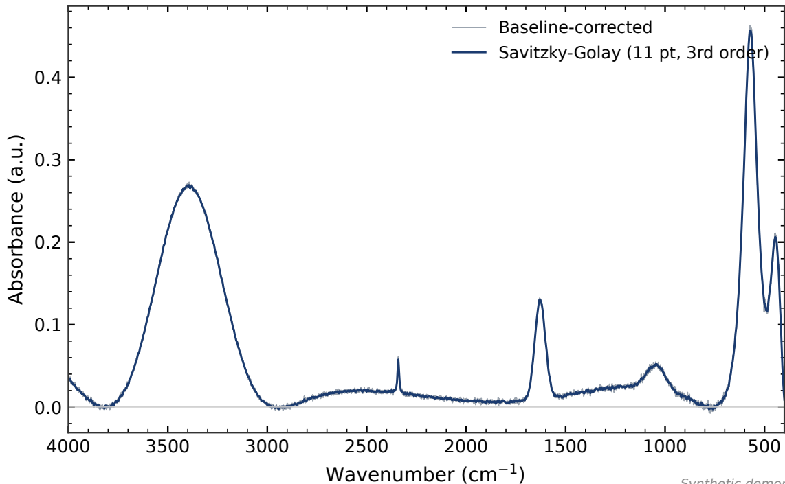
Figure 7. Baseline-corrected synthetic FTIR spectrum
