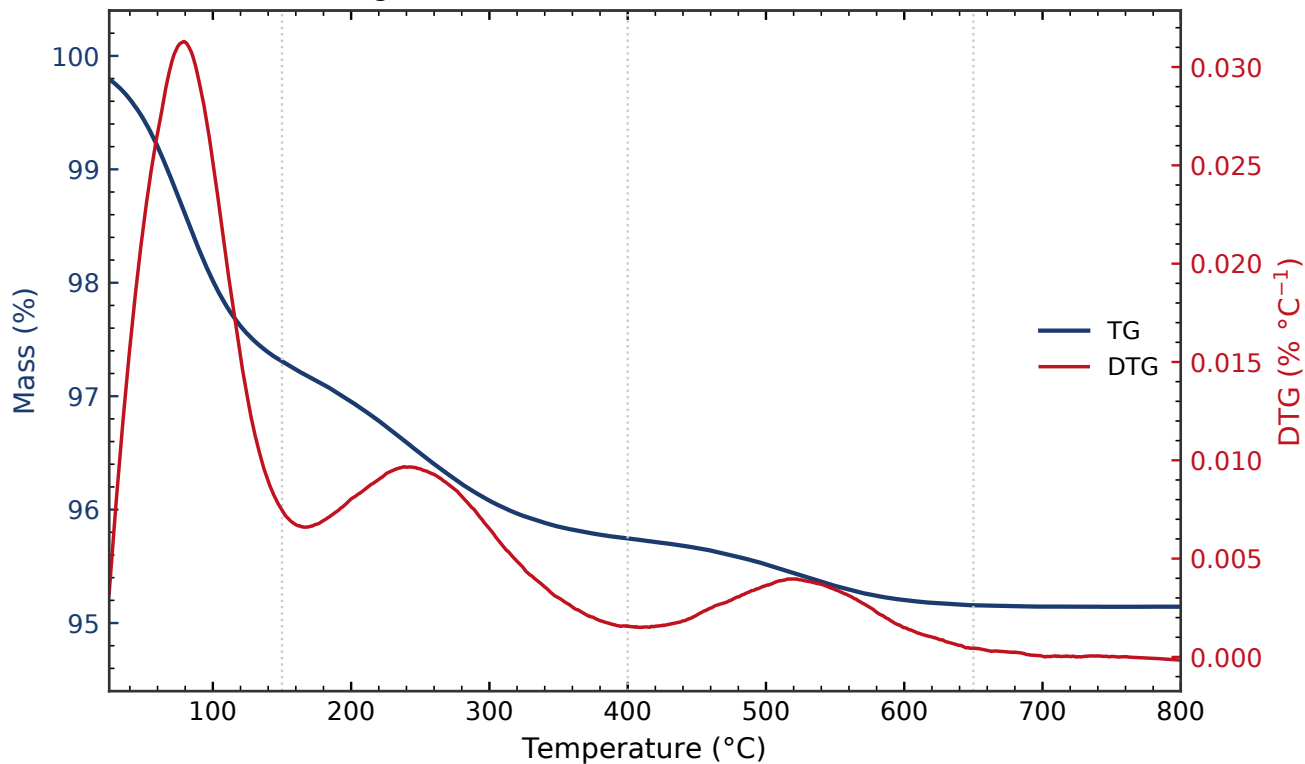
Figure 16. Combined TG and DTG traces
