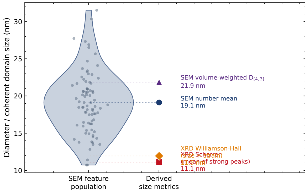
Figure 17. Why XRD and SEM sizes differ -- they measure different things
