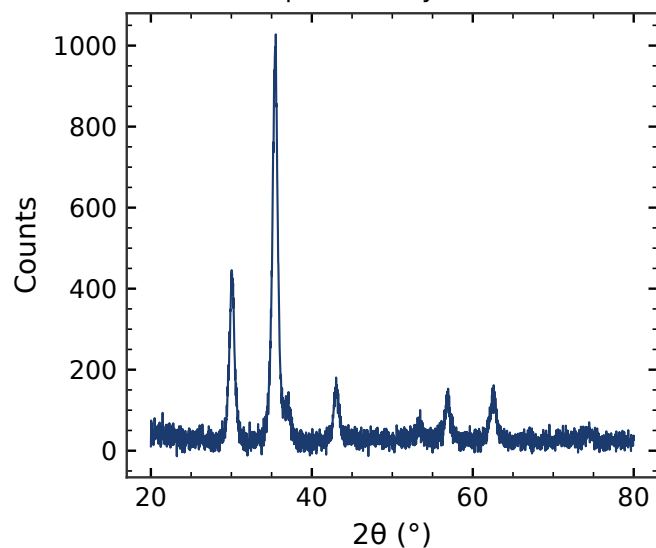
XRD - phase & crystallite size
