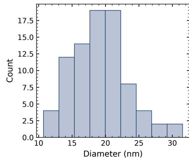
SEM - size distribution
