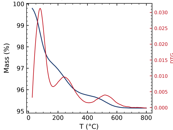
TGA / DTG - volatile content
