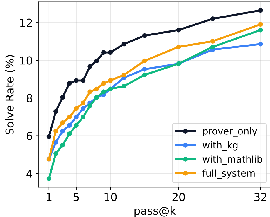
PutnamBench
