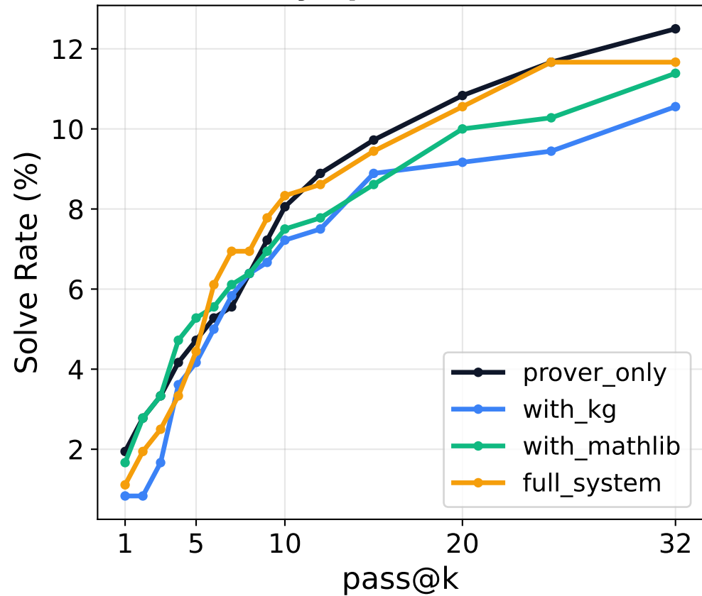
MathOlympiadBench (360)
