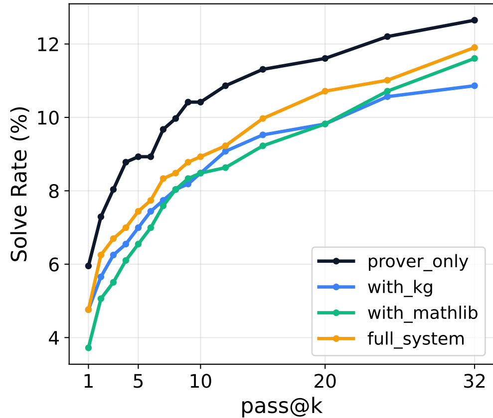
PutnamBench (672)
