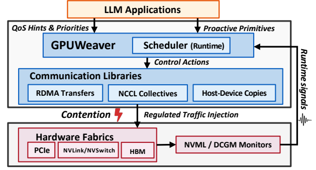
Figure 6: System overview of GPUWeaver.
