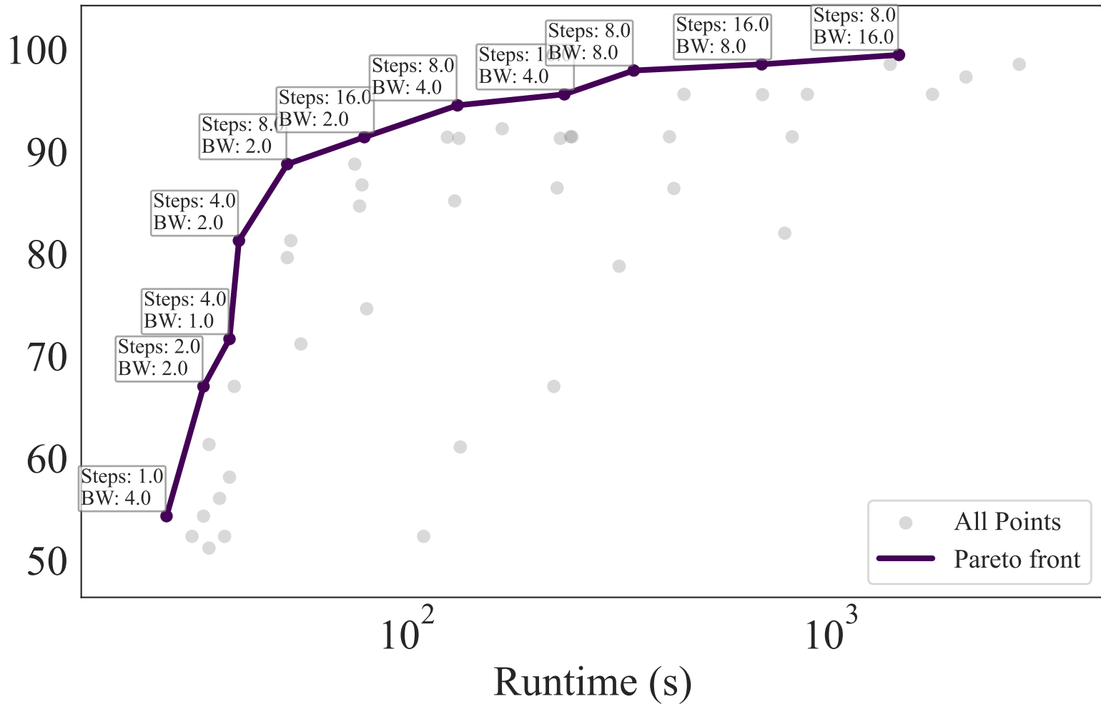
Pareto front of BLEU Score vs Runtime
