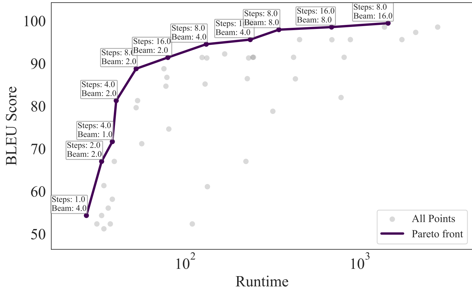
Pareto front of BLEU Score vs runtime
