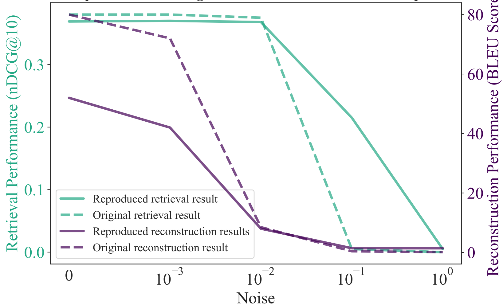
Comparison of nDCG@10 and BLEU Score with noise injection
