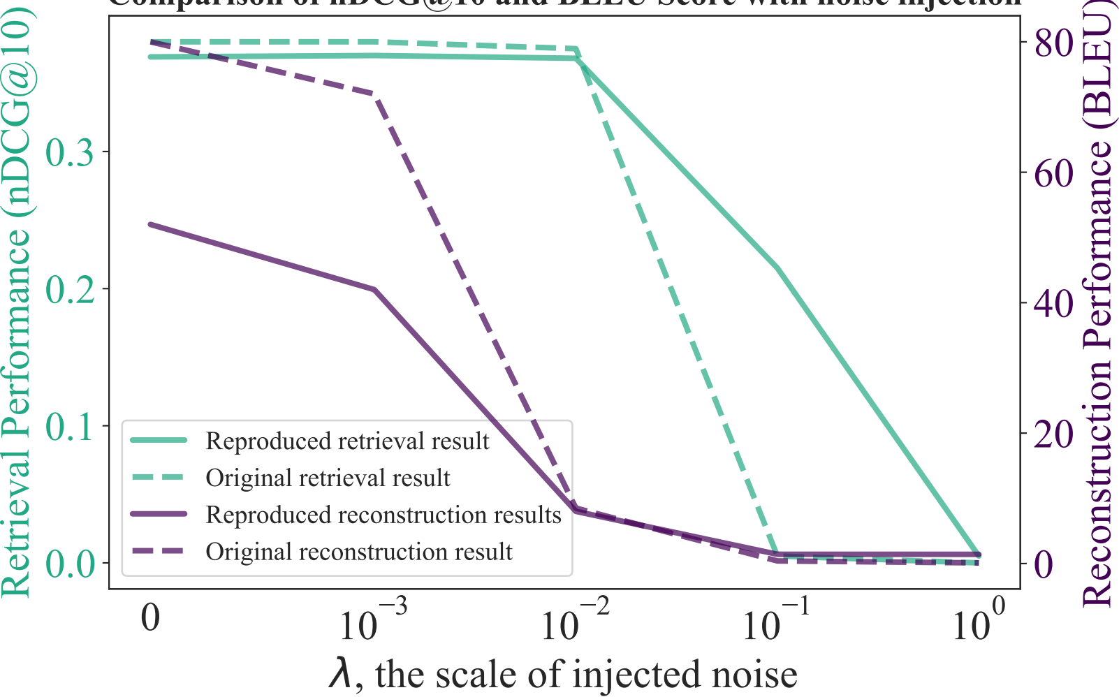
Comparison of nDCG@10 and BLEU Score with noise injection
