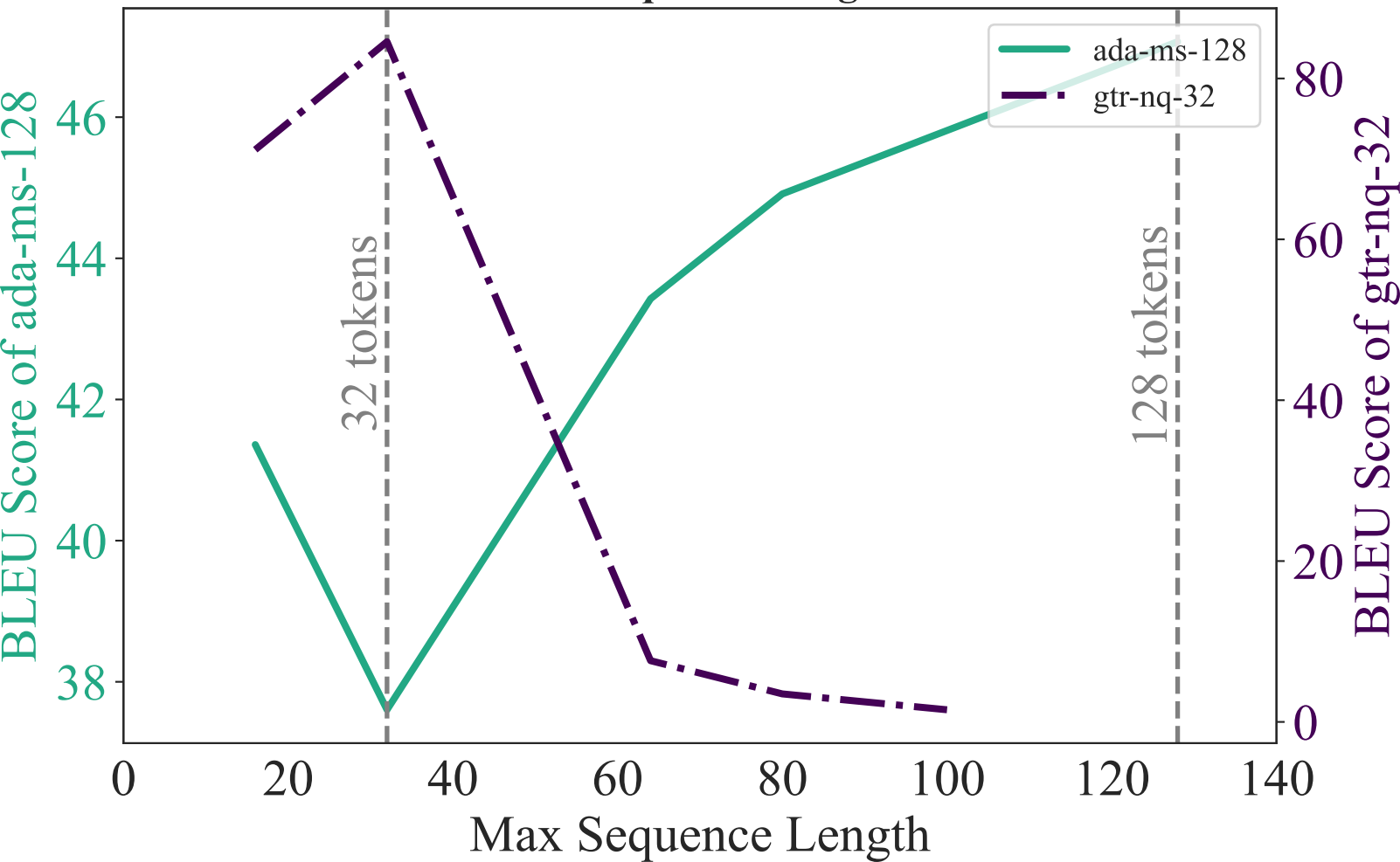
BLEU Score vs Max Sequence Length for Two Models
