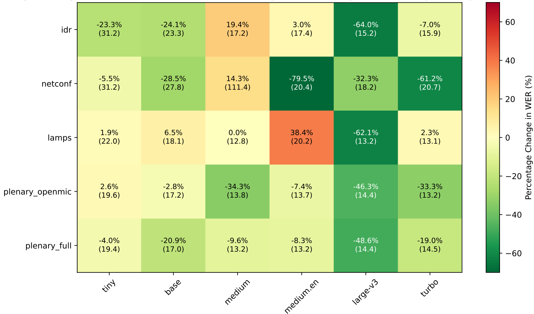
Percentage Change in WER and Absolute WER for no-prev-text mitigation technique compared to baseline
