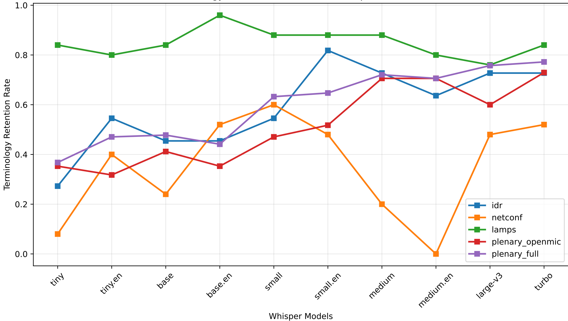
Terminology Retention Rate across Whisper Model Sizes
