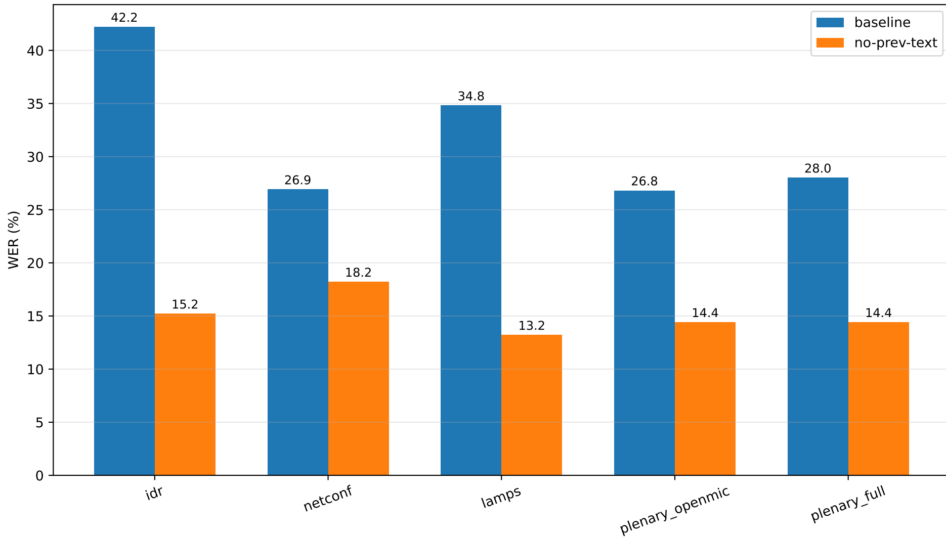
WER for large-v3 model with baseline and no-prev-text mitigation technique
