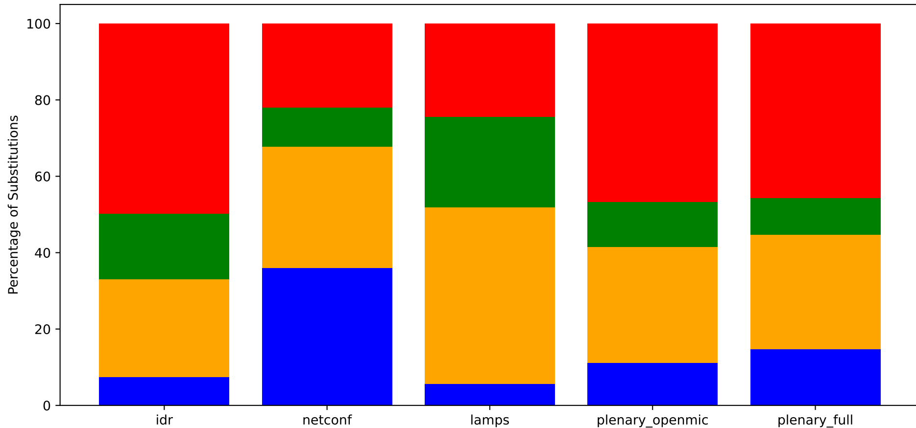
Substitution Error Breakdown (Auto Transcription),average
