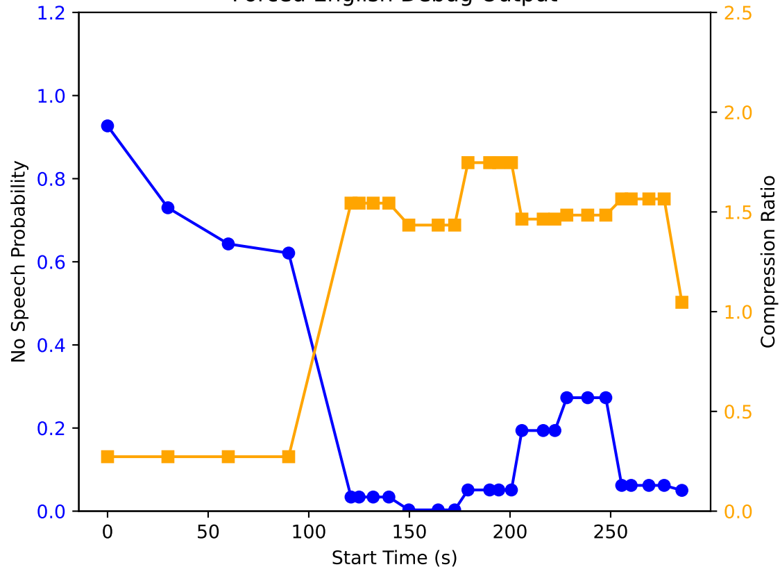
Forced English Debug Output
