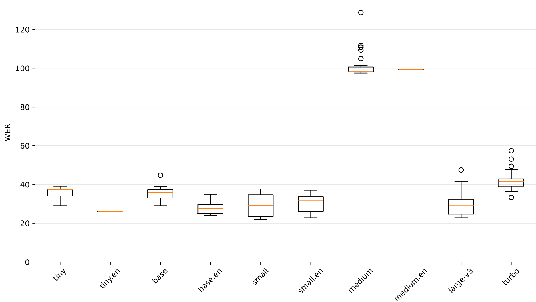
WER distribution
