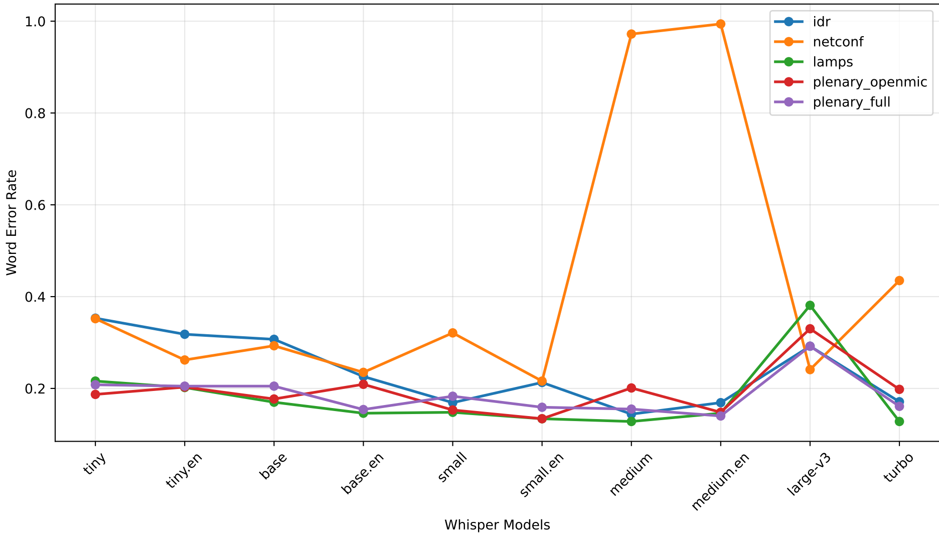
WER across Whisper Model Sizes
