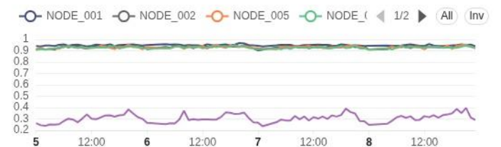
PDP Setup SR Without Roaming
