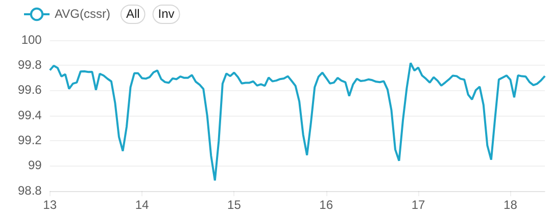
Voice Call Success Rate (CSSR)
