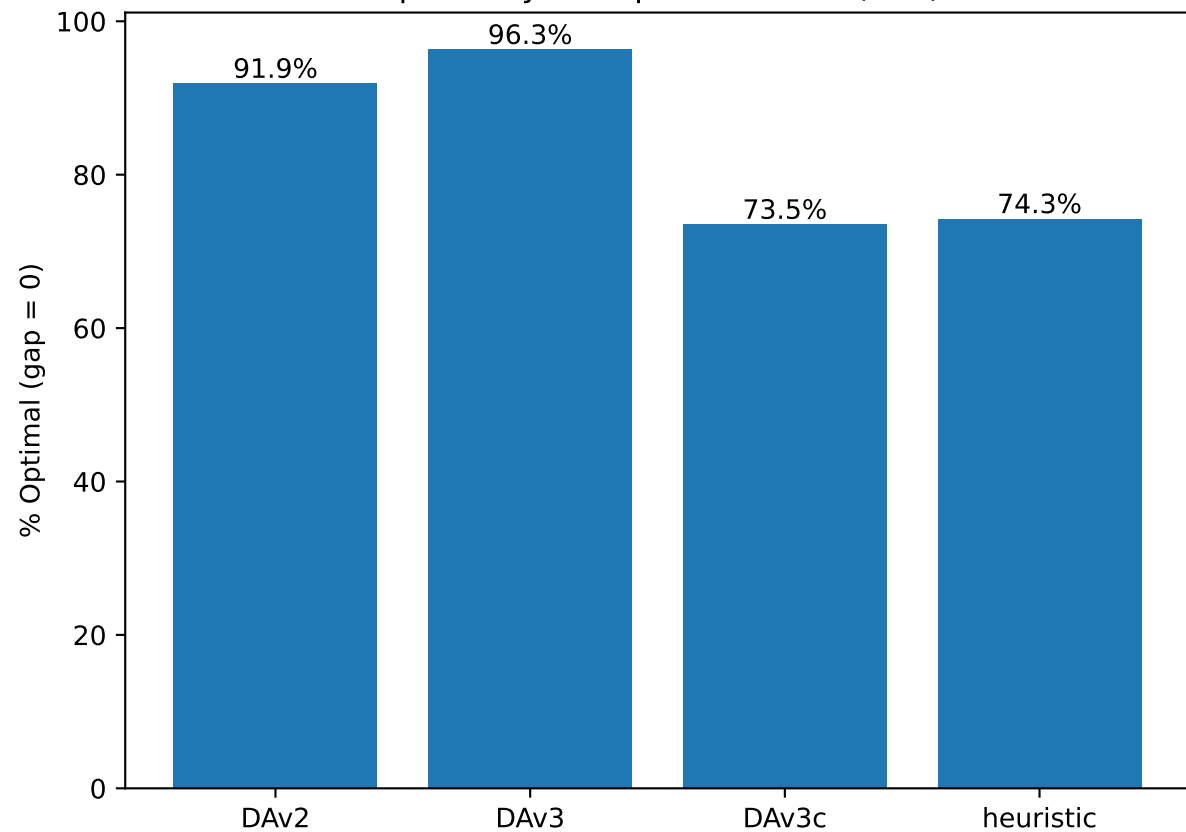
Optimality Rate per Solver n=(136)
