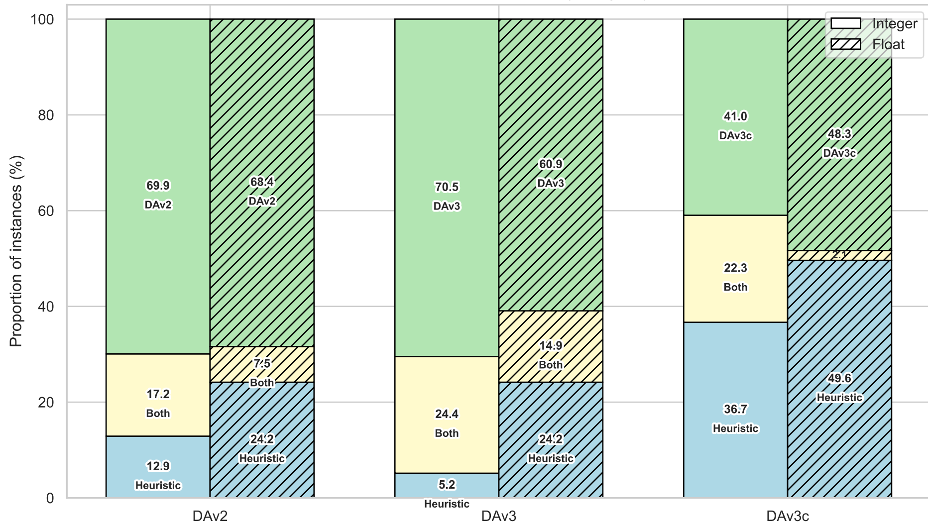
DA Solvers vs MQLib Heuristics by Weight Type
