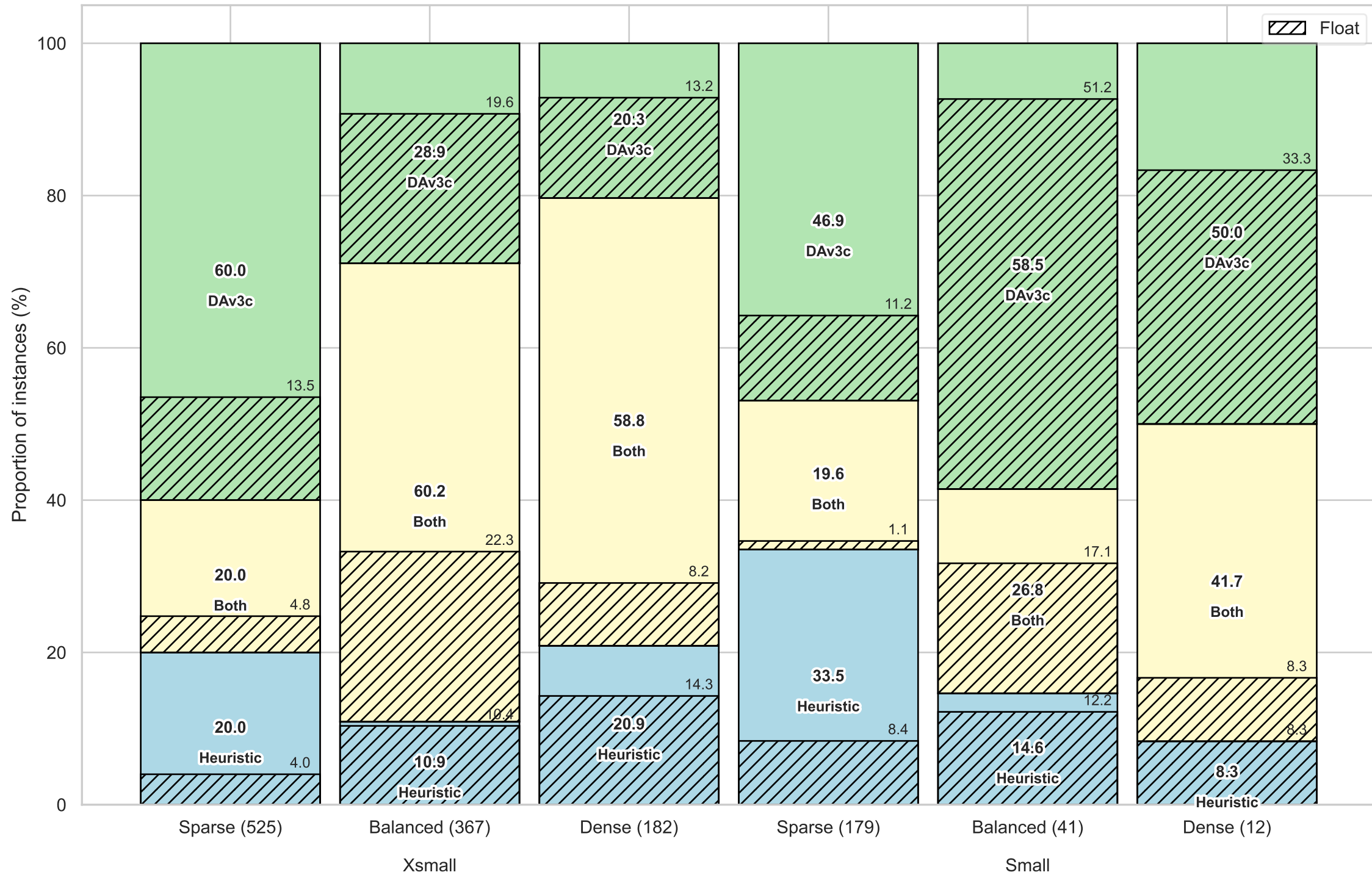
DAv3c vs MQLib Heuristics per Category
